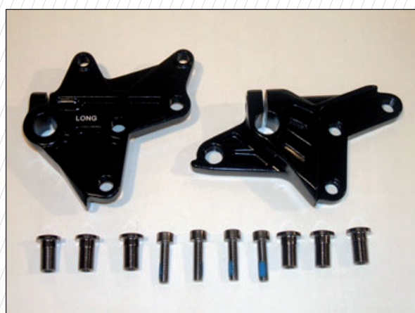
210004 Dropout IDS 12mm Long +10mm No axle
