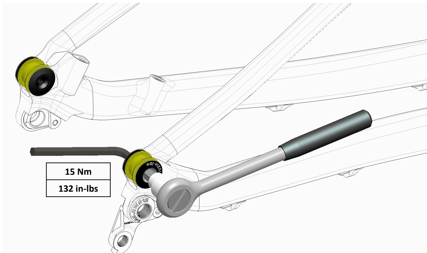
Torque Wrench
