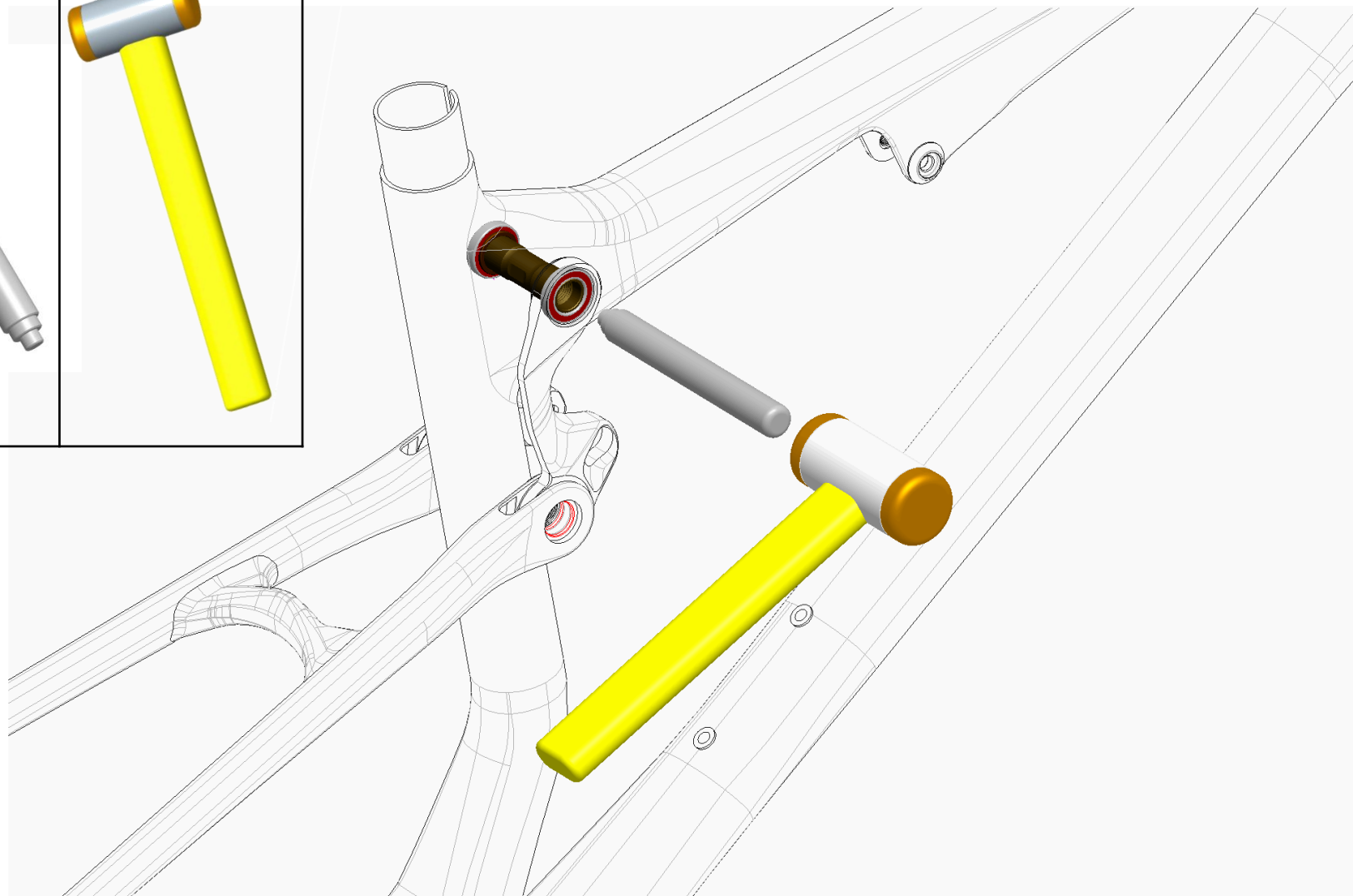
Nylon Hammer
