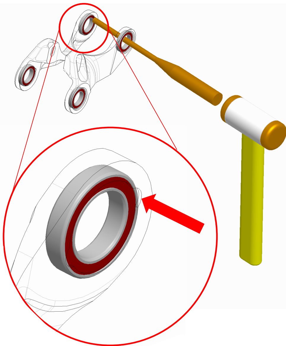
Bearing Punch
