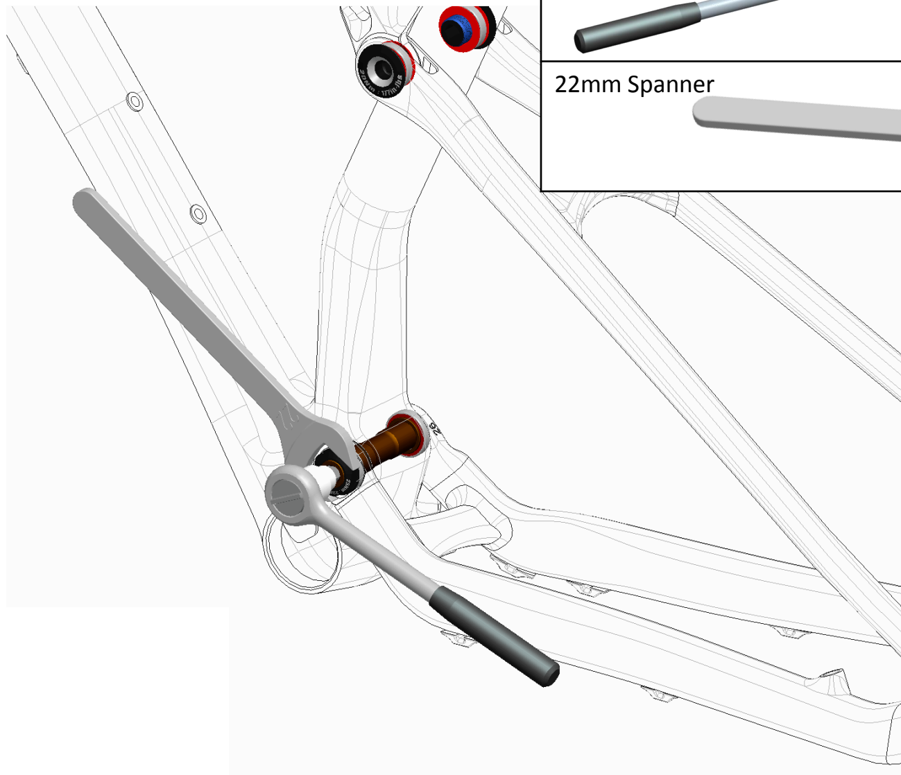
Torque Wrench
