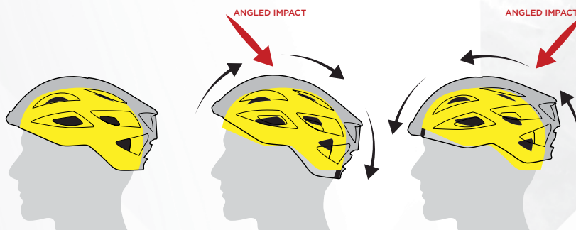
UNDER ANGLED IMPACT THE HELMET SLIDES ON THE MIPS LOW FRICTION LAYER MINIMIZING THE ROTATIONAL VIOLENCE TRANSFERRED TO THE BRAIN
