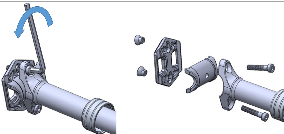
JD-YSP15 Cartridge replacement - Disassembly procedure
