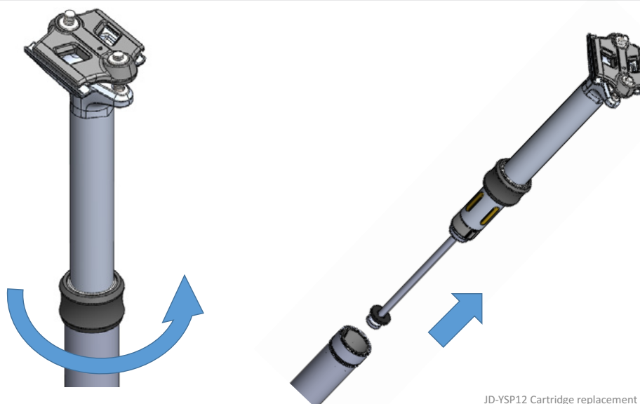
JD-YSP12 Cartridge replacement - Disassembly procedure
