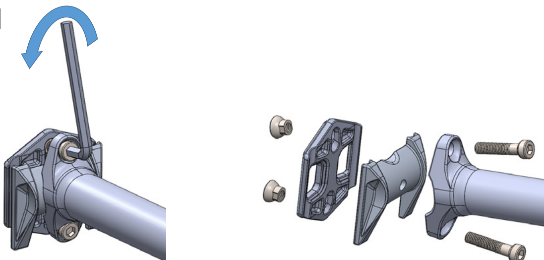
JD-YSP12 Cartridge replacement - Disassembly procedure
