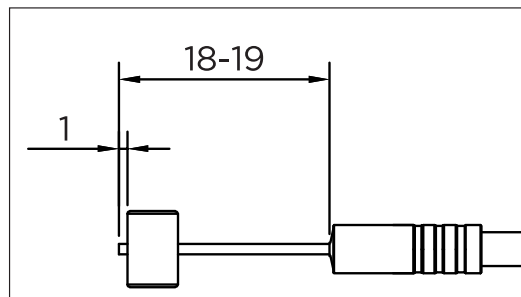
6. Assemble the nut and screw set with the cable; measure the length of the cable 18-19mm from the cable cap to the end of cable, leave about 1mm end of cable, then screw the nut with a 2mm allen key.
