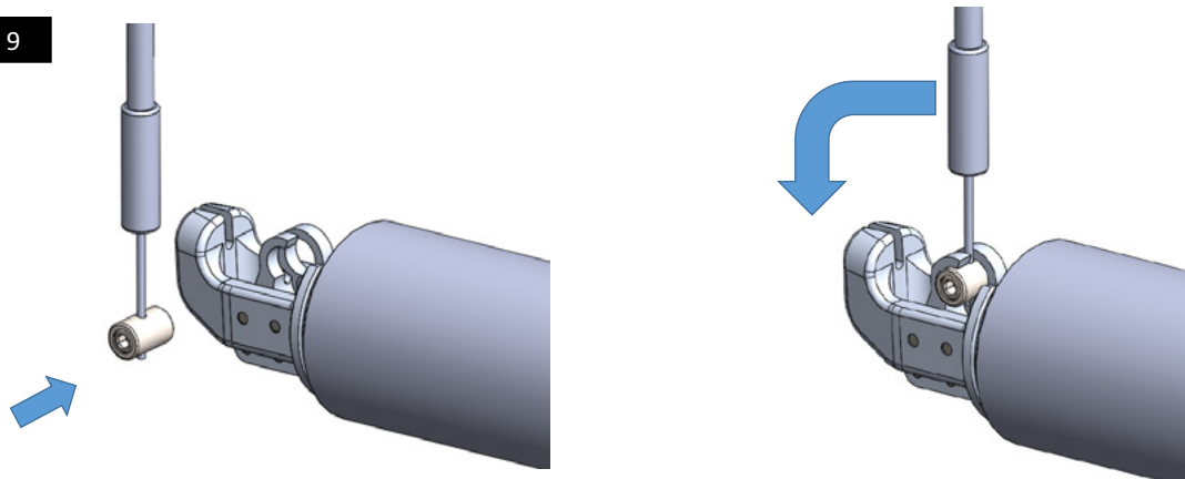
JD-YSP15 Cartridge replacement - Assembly procedure
