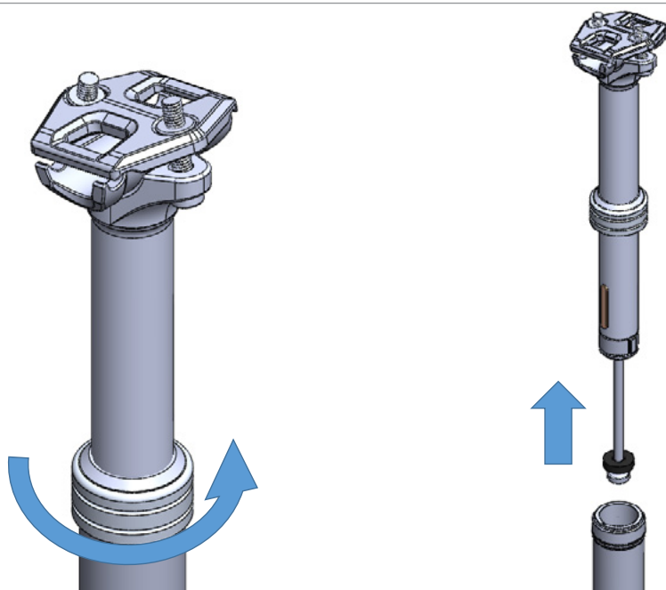
JD-YSP15 Cartridge replacement - Disassembly procedure
